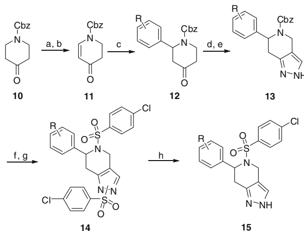
Scheme 4. Reagents and conditions: (a) Br_2 , ethylene glycol; (b) DBU, DMSO, 85 °C, then HCl; (c) CuBr \cdot SMe_2 , BF_3 \cdot OEt_2 , THF, Grignard reagent; (d), HCO_2Et , NaOH, PhH, MeOH; (e) N_2H_4 \cdot H_2O , MeOH, rt; (f) HBr, DCM or Pd/C, H_2 , MeOH; (g) pyridine, 4-chlorobenzenesulfonyl chloride; (h) NaOH, THF, H_2O .
