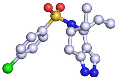
Figure 2. Compound 37 (inactive enantiomer).
