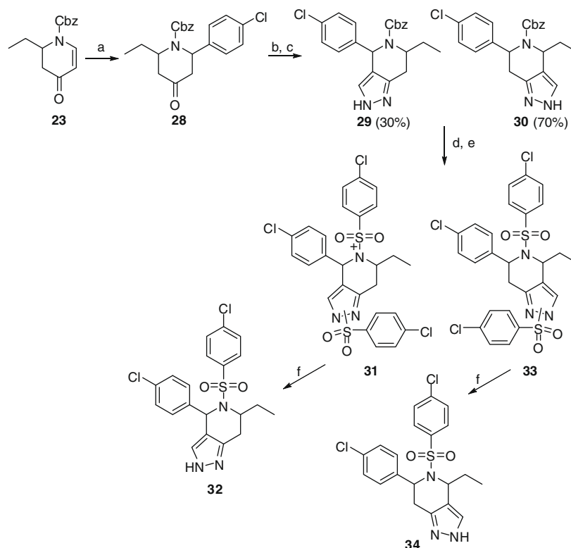
Scheme 7. Reagents and conditions: (a) 4-chlorophenylmagnesium bromide, CuBr·SMe 2 , BF 3 ·OEt 2 ; (b) NaH, HCO 2 Et, MeOH, PhH; (c) N 2 H 4 ·H 2 O; (d) TMSI, CH 3 CN; (e) 4-chlorobenzenesulfonyl chloride.
