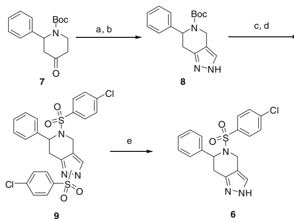
Scheme 3. Reagents and conditions: (a) HCO_2Et , NaH, MeOH, PhH; (b) N_2H_4 \cdot H_2O , MeOH, rt; (c) TFA, rt; (d) 4-chlorobenzenesulfonyl chloride, pyridine; (e) NaOH, THF, H_2O .
