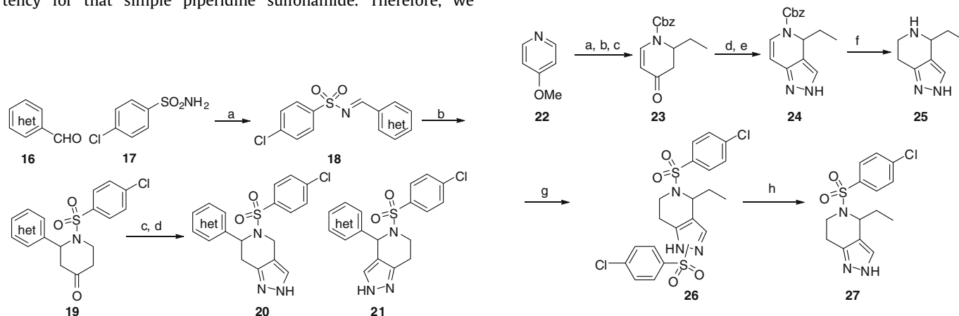
Scheme 6. Reagents: (a) CbzCl, PhMe; (b) EtMgBr, THF; (c) HCl; (d) DMF–DMA; (e) N 2 H 4 ·H 2 O, HOAc; (f) Pd/C, H 2 , MeOH; (g) pyridine, 4-chlorobenzenesulfonyl chloride; (h) NaOH, THF, H 2 O.
